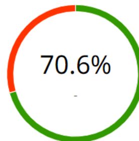
Semantic Analysis
